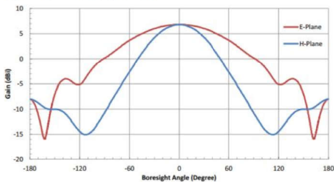
Typical Antenna Pattern @ 115 GHz
