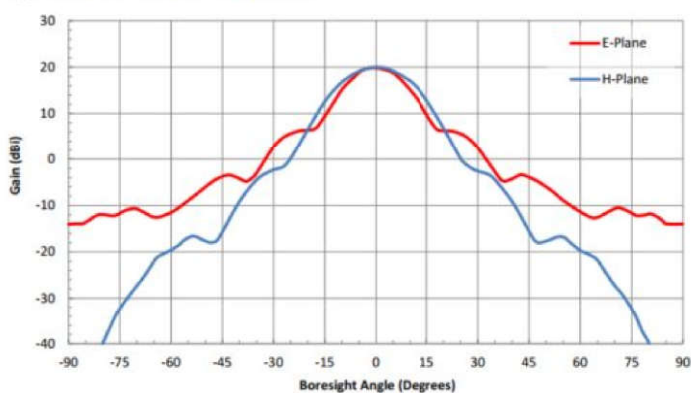
Typical Antenna Pattern @ 93.5 GHz
