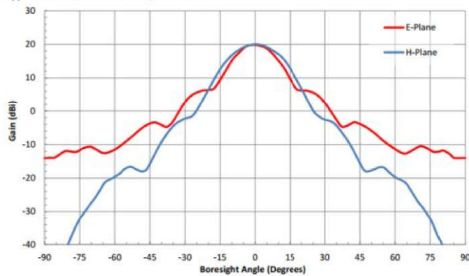
Typical Antenna Pattern @ 82 GHz
