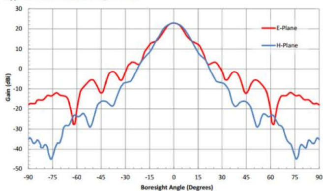
Typical Antenna Pattern @ 63 GHz
