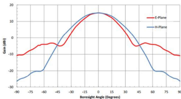
Typical Antenna Pattern @ 25.25 GHz
