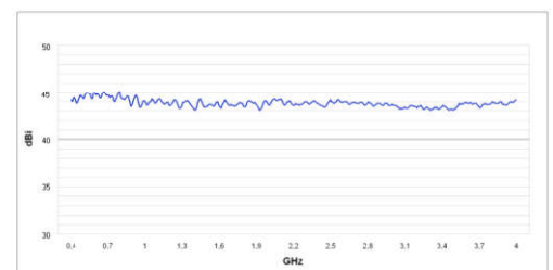
Gain diagram
