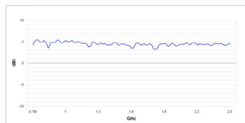
Gain diagram
